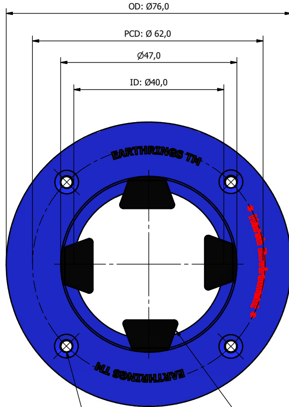
Front View ( 1.5 : 1 )
